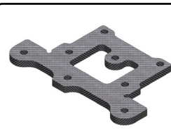
C-00180-003 Steering Top Plate - Graphite 2mm - 1 pc
